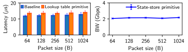
(a) Latency overhead of (b) Bandwidth overhead of lookup table primitive.
